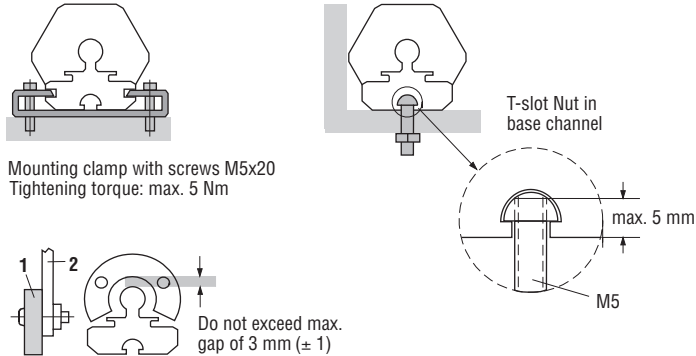
1 U-Magnet 2 Mounting plate and screws non-ferrous material
