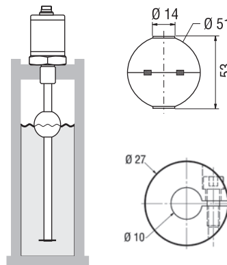
Magnet float (upon request) Part no. 251 447 - Density 720 kg/m 3 - Material 1.4571 polished AISI 316 Ti - Pressure < 25 bar
