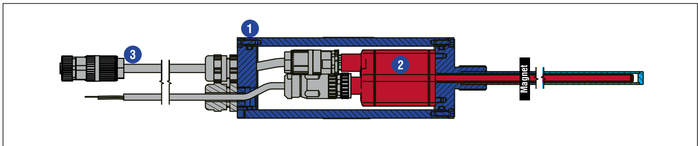
Fig. 3: Structure of RM5 EtherNet/IP™
